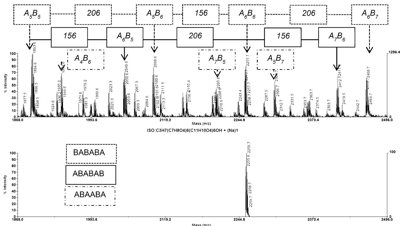
Figure 3. Details of the MALDI-ToF MS of a P(\text{MLA}^{\text{Bz-alt-MLA}})^{\text{All}} prepared by simultaneous ROP of (S)\text{-MLA}^{\text{Bz}} and (R)\text{-MLA}^{\text{All}} with 1d in presence of 1 equiv of i PrOH (Table 2, entry 4) using IAA as matrix. The major populations correspond to macromolecules ionized by \text{Na}^+ (see the simulated spectrum at the bottom of the figure) and to alternating copolymers with \text{MLA}^{\text{Bz}} (B) as the first unit (dashed line), alternating copolymers with \text{MLA}^{\text{All}} (A) as the first unit (solid line), and copolymers with one alternation error (dashes/dotted line).
